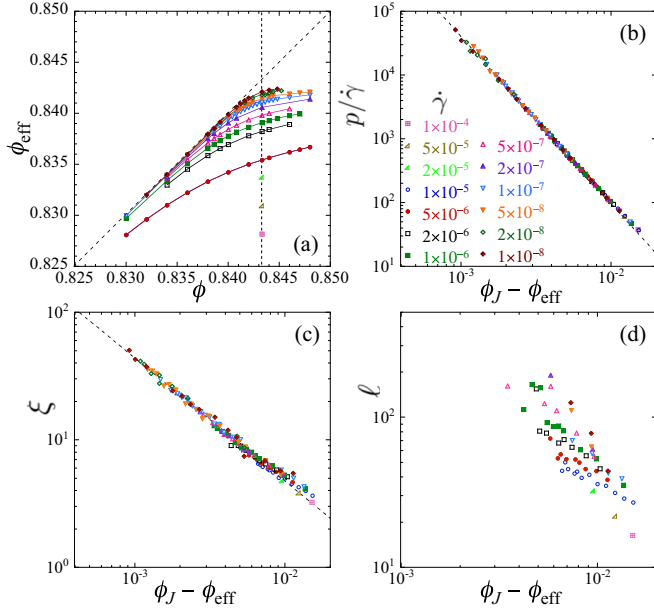
FIG. 10. (a) Effective packing \phi_{\text{eff}}(\phi, \dot{\gamma}) = \phi - cE^{1/2y} vs \phi for different strain rates \dot{\gamma} ; the diagonal dashed line denotes \phi_{\text{eff}} = \phi , while the vertical dashed line locates \phi_J \approx 0.8433 . (b) p/\dot{\gamma} vs \phi_J - \phi_{\text{eff}} , (c) \xi vs \phi_J - \phi_{\text{eff}} , and (d) \ell vs \phi_J - \phi_{\text{eff}} , for different strain rates \dot{\gamma} . The value \phi_J = 0.8433 is used in making these plots. In (b) and (c) the dashed line is a power-law fit to the data for \phi_J - \phi_{\text{eff}} \leq 0.005 and gives the exponent \beta = 2.62 for p/\dot{\gamma} and \nu = 0.98 for \xi . The symbols in (a), (c), and (d) follow the same legend as in (b).
