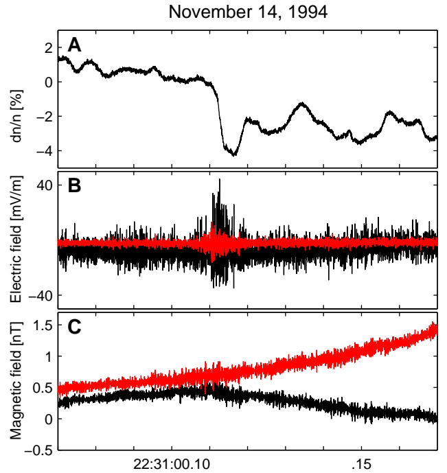
Fig. 1. Panel A shows the density variations observed along the satellite trajectory (perpendicular to \mathbf{B}_0 ). The two recorded electric wave field components are shown in panel B. The black and red lines are the most perpendicular and the most parallel \mathbf{E} -field component respectively. For both components we note a clear enhancement associated with the density gradient. In panel C corresponding magnetic wave fields are presented. Here the spin axis component (black line) has an angle of 77° to \mathbf{B}_0 and the spin plane component (red line) has an angle of 43° to \mathbf{B}_0 . The increase in the magnetic wave activity is barely visible.
