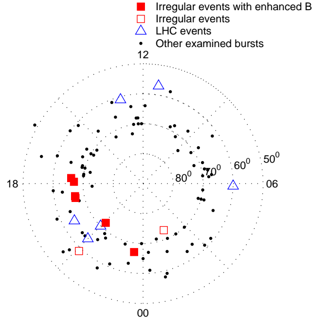
Fig. 8. View over the northern hemisphere. The time is given in MLT and the circles indicate the latitude. Due to the 63^\circ inclination of the Freja orbit we do not measure above 75^\circ . Irregular density variation events are marked by squares. The filled squares indicate where events with enhanced magnetic wave activity has been found. Triangles denote LHC events, while dots mean that no density variations are detected. Event 1, that includes both irregular density variations and LHCs, is marked by a filled square.
