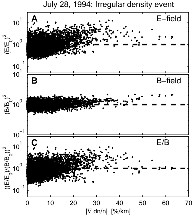
Fig. 4. Variations of the wave power for an irregular density variation case. The analysis is based on 10 seconds of data from July 28, 1994, containing the three gradients presented in Fig. 3. Panel A and B show variations in the electric and magnetic wave power versus the gradient of the density, |\nabla dn/n| . The wave power is normalized to the average wave power over the surrounding 0.5 s. Hence, a ratio larger than one means that there is an enhancement in the wave power. For steep gradients ( |\nabla dn/n| \gtrsim 30 %/km) we see clear enhancements of both the electric and the magnetic wave power. Panel C presents the variation in E/B versus |\nabla dn/n| .
