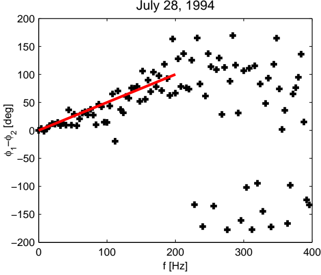
Fig. 6. Phase difference versus frequency for two cross correlated density signals. The phase difference is small in the zero frequency limit. For low frequencies (long wavelengths) there is a good fit to a straight line, and the estimated phase velocity is just the satellite velocity with respect to Earth. The linear fit is made for data with a coherence above 0.5. Hence, we conclude that the density variations are spatial structures down to scale lengths of a few ion gyroradii ( \rho_{H^+} = 5\text{--}10 m, \rho_{O^+} = 20\text{--}40 m). Data is taken from the same interval as the data shown in Fig. 3.
