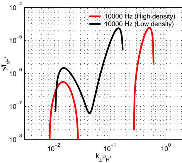
Fig. 11. The temporal growth rate versus k_{\perp} \rho_{H^+} ( \rho_{H^+} = 7 m). In both the high (red lines) and low density (black line) cases there are two peaks in growth rate, one at the perpendicular wave vector where we believe most of the wave energy to be located and one at larger k_{\perp} .
