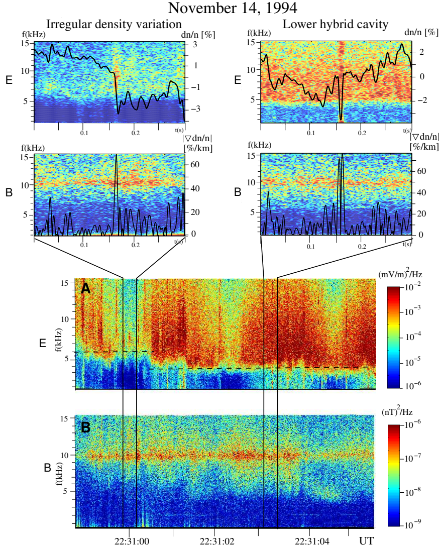
Fig. 2. The two large panels show seven seconds long electric and magnetic field spectrograms from November 14, 1994. At 22:31:00.5 UT the total density changes from 7900 \text{ cm}^{-3} to 3100 \text{ cm}^{-3} . The associated change in the lower hybrid cut-off frequency is marked with dashed lines in panel A. Before the density drop irregular density variations are found and after are LHCs detected. Enlarged are 0.3 seconds from two parts of the burst. The two top-left panels show an irregular density variation event and the two top-right panels show an LHC event.
