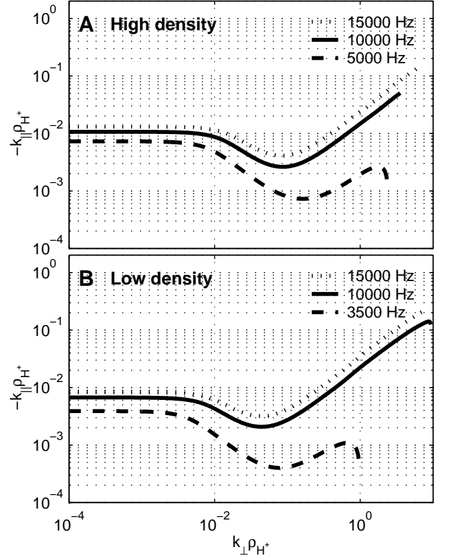
Fig. 9. Constant frequency curves in wave vector space. The parallel and perpendicular wave vectors are normalized to the gyro radius of the 2 eV protons in the models, that is \rho_{H^+} = 7 \text{ m} . Panel A is the results from modelling the high density case, where irregular density events are present. Panel B is the dispersion curves for the low density case. The overall structure is very similar. We can note a small shift of a curve at a given frequency towards larger k for a higher density.
