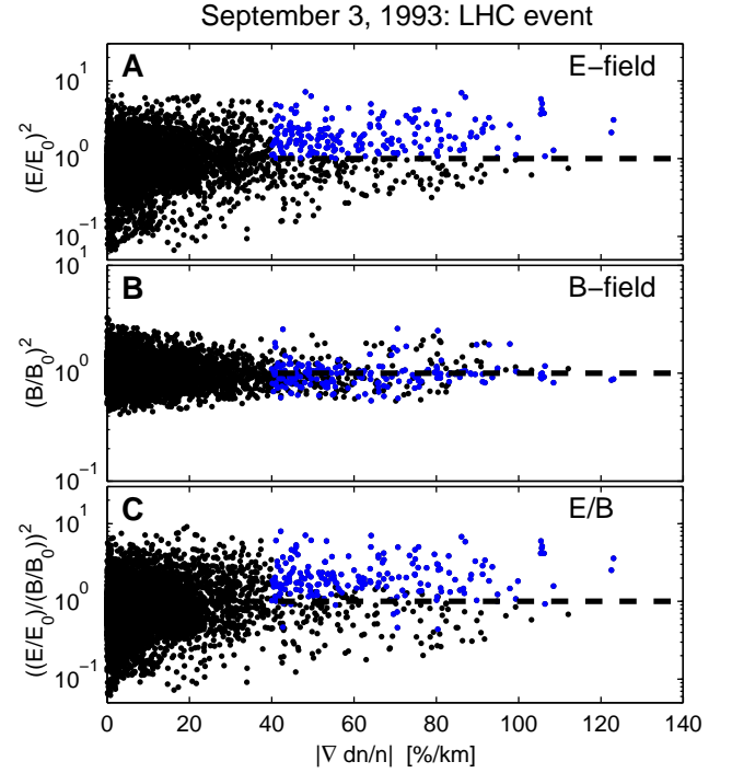
Fig. 5. Variations of the wave power for a LHC case. The analysis is based on 10 seconds of data observed on September 3, 1993. Analysis and panels are the same as in Fig. 4. All points with enhanced electric wave power and |\nabla dn/n| \gtrsim 40 %/km are colored blue. From panel B we then see that there is no correlation between enhancements in the electric power and enhancements in the magnetic power.
