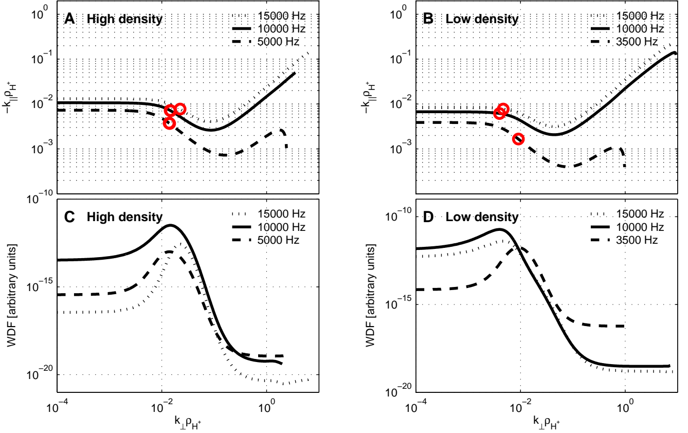
Fig. 10. The peaks in the reconstructed WDF are presented on top of constant frequency curves in wave vector space in panels A and B. In panels C and D the WDF is plotted versus normalized k_{\perp} . As before \rho_{H^+} = 7 m.
