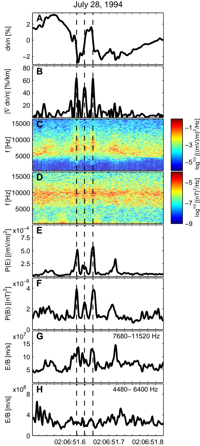
Fig. 3. Panel A shows the density profile. Panel B displays the absolute value of the gradient of the density. We assume spatial structures and the gradient is given in %/km. The electric and magnetic power spectral densities are plotted versus time and frequency in panels C and D. The electric and magnetic wave powers in the frequency range 7680–11520 Hz are given in panels E and F. Panels G and H present E/B for the two frequency intervals 7680–11520 Hz and 4480–6400 Hz.
